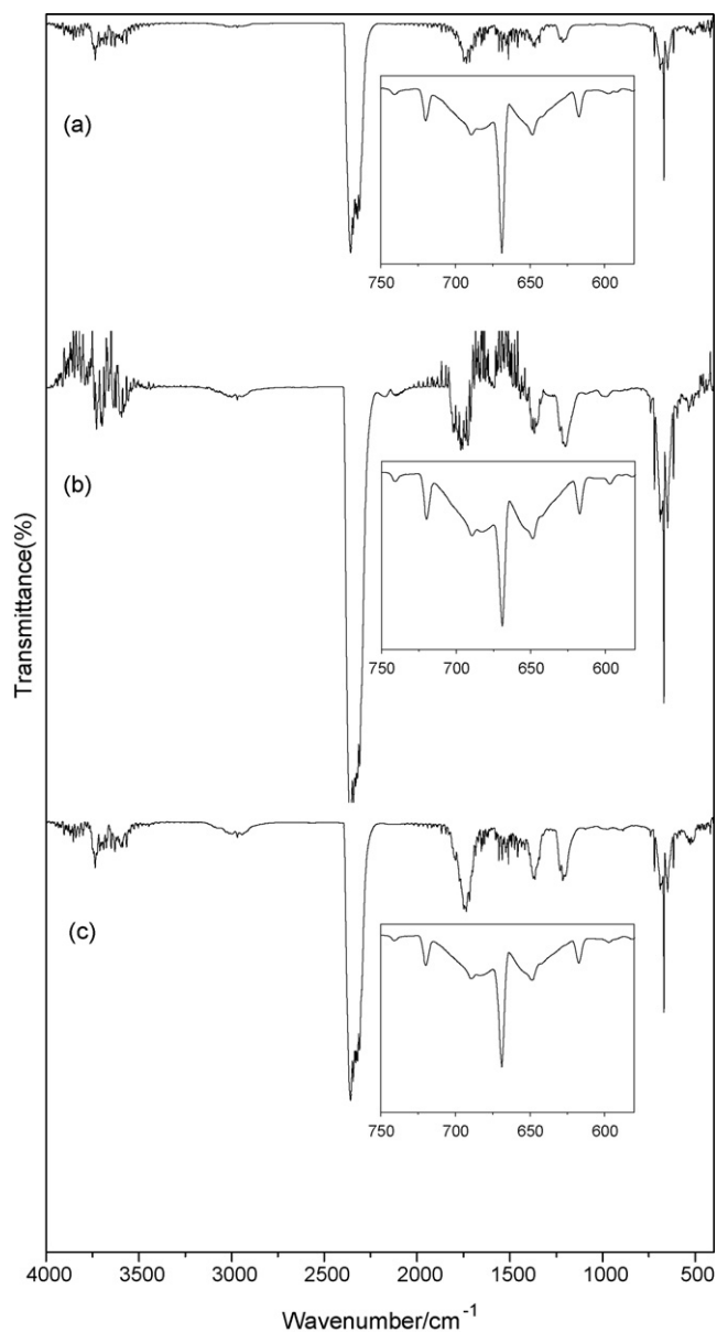
Fig. 5. IR spectra of gaseous products evolved during the decomposition of the compounds: (a) \text{Na}_2\text{L}\cdot\text{H}_2\text{O} , (b) \text{CoL}\cdot 2\text{H}_2\text{O} (c) \text{ZnL}\cdot 2\text{H}_2\text{O} . L = malonates.
