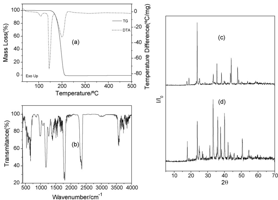
Fig. 1. Study of thermal behaviour of malonic acid: (a) simultaneous TG-DTA curves ( m = 10.744 \text{ mg} ), (b) IR spectrum of the gases released during the decomposition of malonic acid, (c) X-ray powder diffraction pattern and (d) X-ray powder diffraction pattern of the malonic acid heated until 125^\circ\text{C} .
