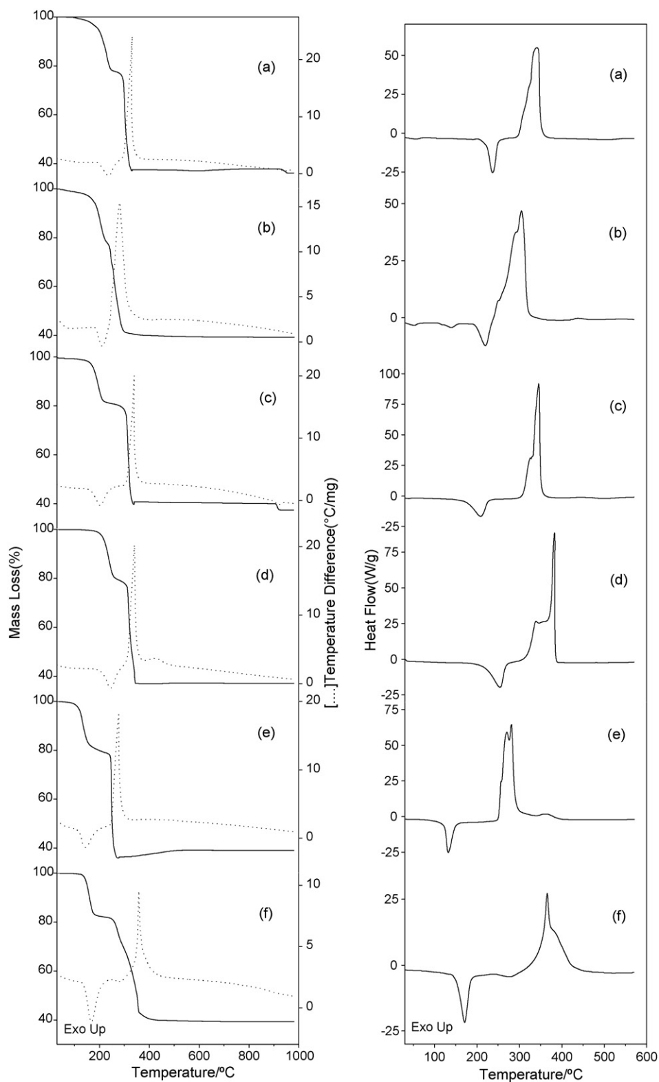
Fig. 4. Simultaneous TG-DTA and DSC curves of the compounds: (a) \text{MnL}_2 \cdot 2.5\text{H}_2\text{O} ( m = 7.441 and 2.032 mg), (b) \text{FeL}_2 \cdot 2.5\text{H}_2\text{O} ( 7.327 and 2.011 mg), (c) \text{CoL}_2 \cdot \text{H}_2\text{O} ( 7.424 and 2.034 mg), (d) \text{NiL}_2 \cdot \text{H}_2\text{O} ( 7.232 and 2.021 mg), (e) \text{CuL}_2 \cdot \text{H}_2\text{O} ( 7.151 and 2.028 mg) and (f) \text{ZnL}_2 \cdot \text{H}_2\text{O} ( 7.182 and 2.055 mg).
